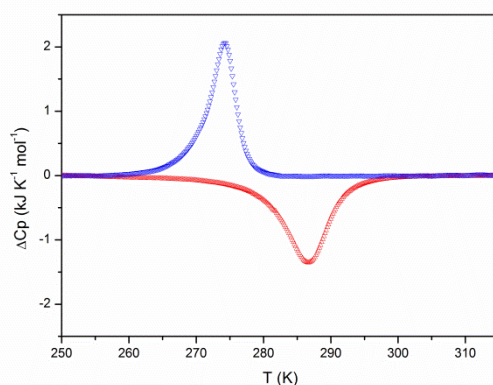
Figure 2. Differential scanning calorimetry (DSC) for 1 upon cooling (▼) and heating (▲) at 10 \text{ K}\cdot\text{min}^{-1} .
