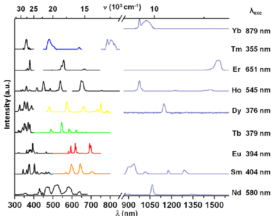
Fig. 22. Normalized solid state excitation and emission spectra for [\text{Ln}_6\text{O}(\text{OH})_8(\text{NO}_3)_6(\text{H}_2\text{O})_n]\cdot 2\text{NO}_3\cdot 2\text{H}_2\text{O} with n = 12 for Ln = Sm-Lu plus Y and n = 14 for Ln = Nd.
