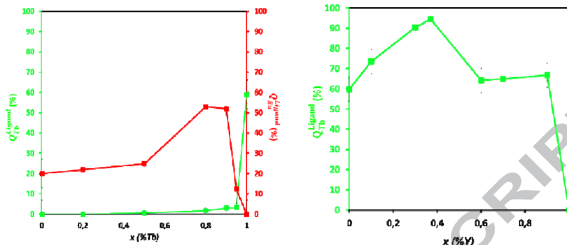
Fig 28. Left: Overall quantum yields Q_{Tb}^{Ligand} and Q_{Eu}^{Ligand} versus x in [Tb_{6x}Eu_{6-6x}O(OH)_8(NO_3)_2(bdc)(Hbdc)_2 \cdot 2NO_3 \cdot H_2bdc]_\infty with 0 \leq x \leq 1 . Right: Overall quantum yields Q_{Tb}^{Ligand} versus x in [Y_{6x}Tb_{6-6x}O(OH)_8(NO_3)_2(bdc)(Hbdc)_2 \cdot 2NO_3 \cdot H_2bdc]_\infty with 0 \leq x \leq 1 .
