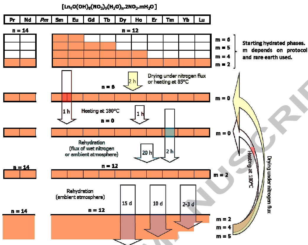
Fig. 21. Relationships between the different crystalline phases of the octahedral hexa-nuclear complexes. Redrawn from reference [138].
