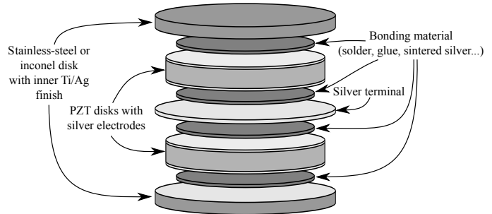
Fig. 1. Exploded view of a vibration sensor. Two vibration elements (PZT ceramics) are used in this device.
