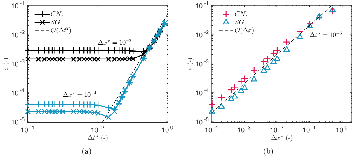
Figure 6. \mathcal{L}_2 error as a function of \Delta t^* for the CN and SG schemes ( \Delta x^* = 10^{-4} ) (a) and \mathcal{L}_2 error as a function of \Delta x^* for the CN and SG schemes ( \Delta t^* = 10^{-5} ).
