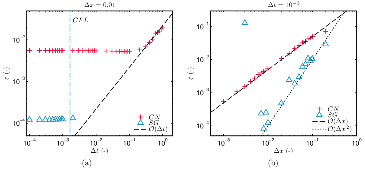
Figure 11. L_2 error \varepsilon for a fixed \Delta x = 10^{-2} as a function of \Delta t (a), and L_2 error \varepsilon for a fixed \Delta t = 10^{-3} as a function of \Delta x .
