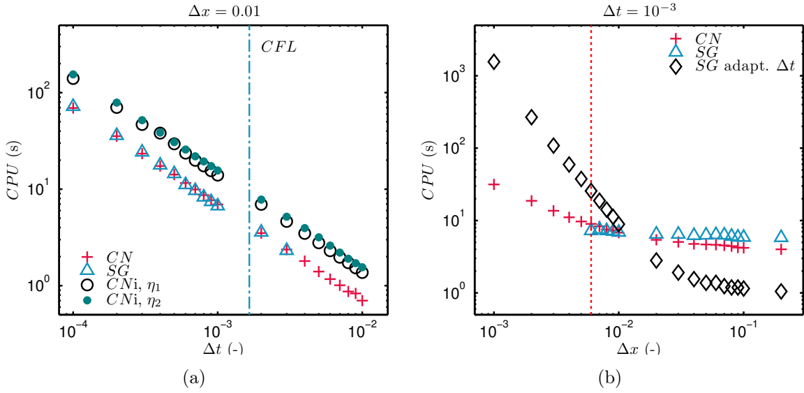
Figure 12. Computational time for \Delta x = 10^{-2} as a function of \Delta t (a), and for \Delta t = 10^{-3} as a function of \Delta x .
