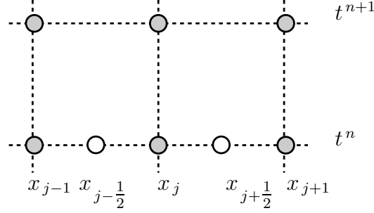
Figure 2. Stencil of the numerical schemes.
