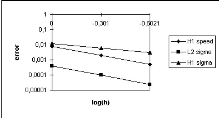
Figure 1: Approximations errors
