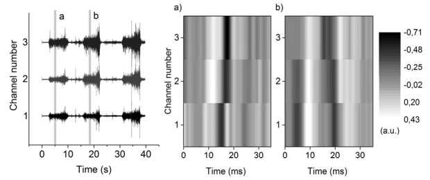
Figure 2. The sEMG recordings x_i . Scaled-up zones a (during little finger extension) and b (index finger extension) are shown. The third movement corresponds to simultaneous extension of little and index finger.
