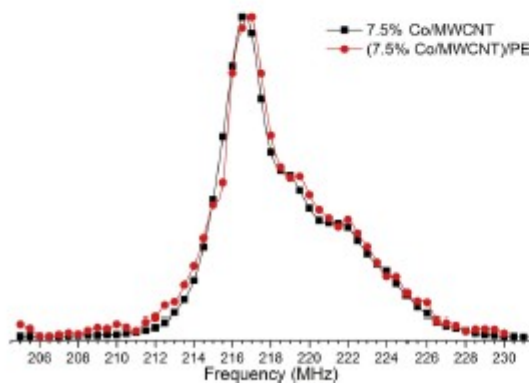
Fig. 8. ^{59}\text{Co} IF-NMR spectra of 7.5% Co/MWCNT hybrid sample after reduction (black squares) and in a PE composite. The spectra coincide within experimental errors proving that the Co is efficiently protected from oxidation in the PE matrix. Note that the 7.5% Co/MWCNT in PE composite contain only 14.7% of Co/MWCNT, i.e. Co content inside the PE composite is only about - 1%. (A colour version of this figure can be viewed online.)
