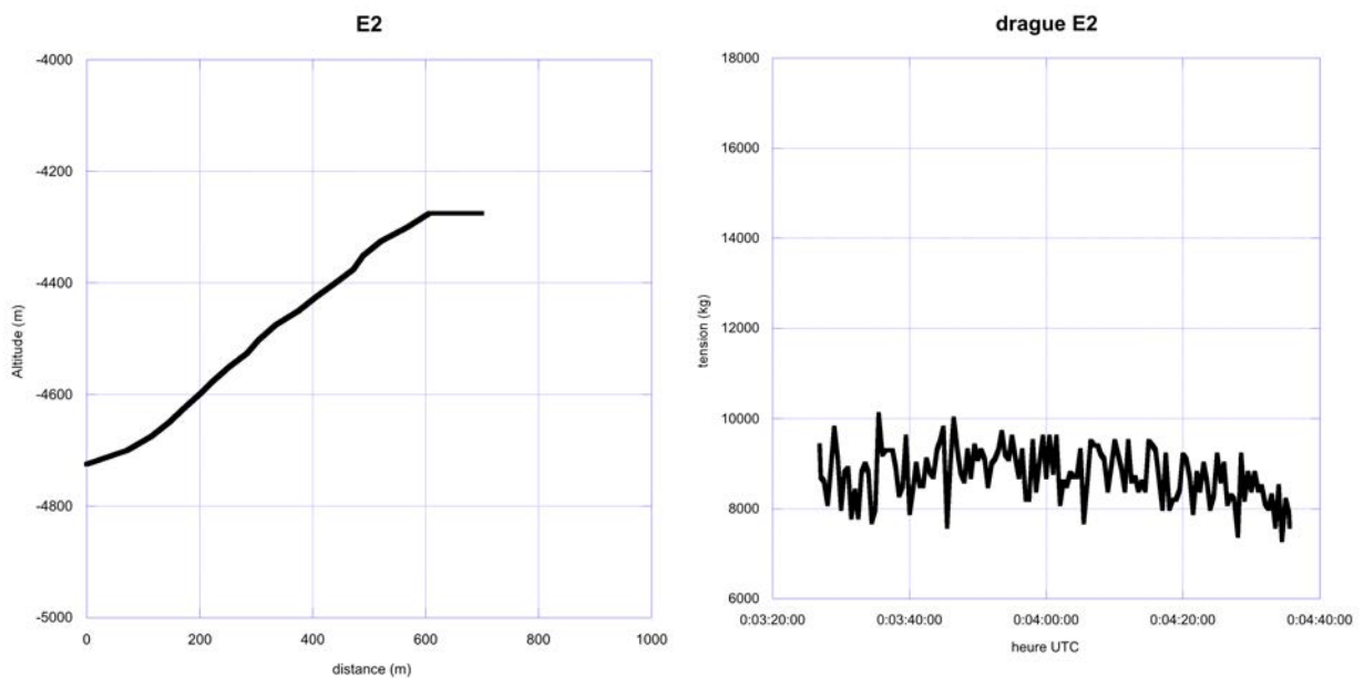
Figure 60: Scheduled bathymetric section for E2 dredge.
