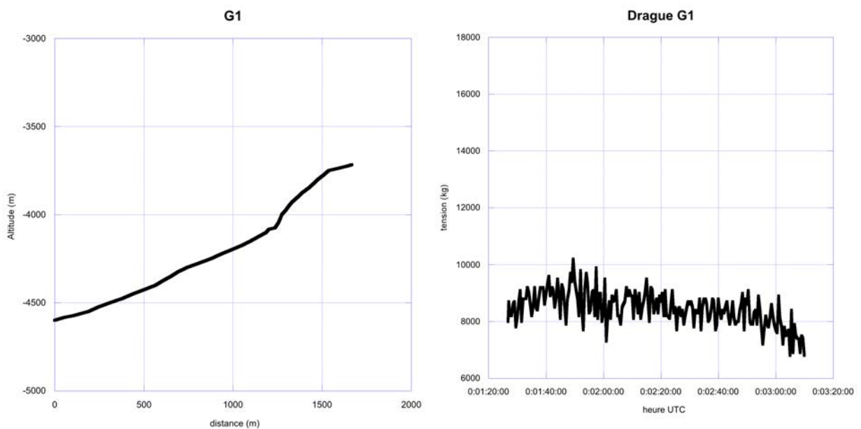
Figure 18: Scheduled bathymetric section for G1 dredge.
