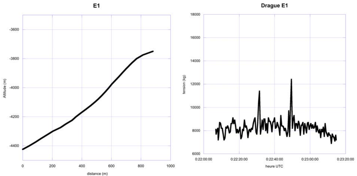
Figure 52: Scheduled bathymetric section for E1 dredge.
