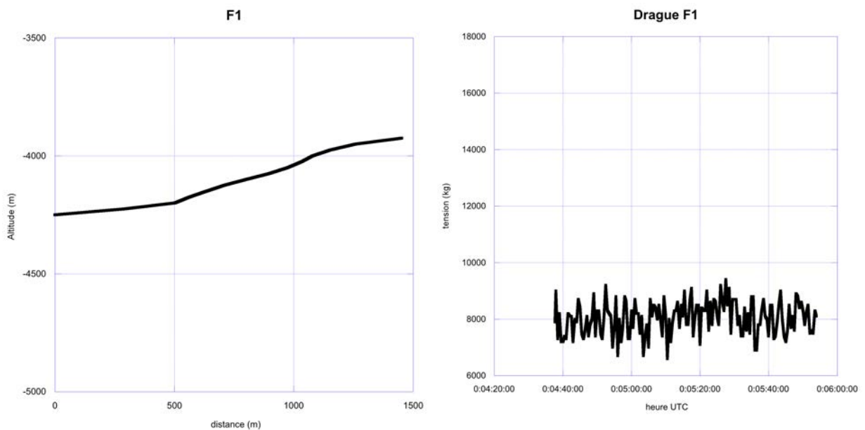
Figure 63: Scheduled bathymetric section for F1 dredge.
