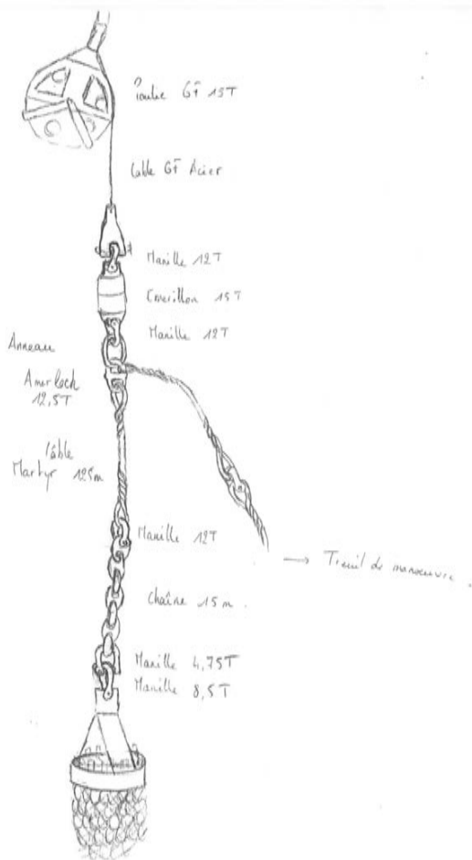
Figure 8: Wiring of the dredge (drawing by Morgane Golain, annotated by Jean Meral). The different parts are not shown at the same scales (cf. figure 9).
