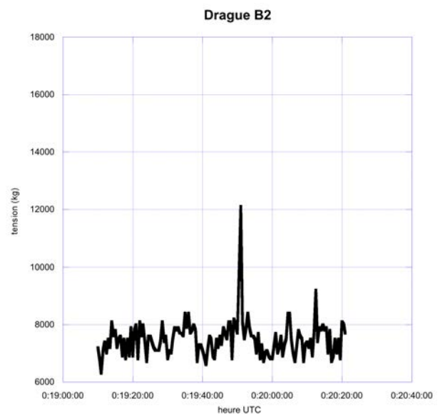
Figure 32: Tension of the cable during dredge B2.
