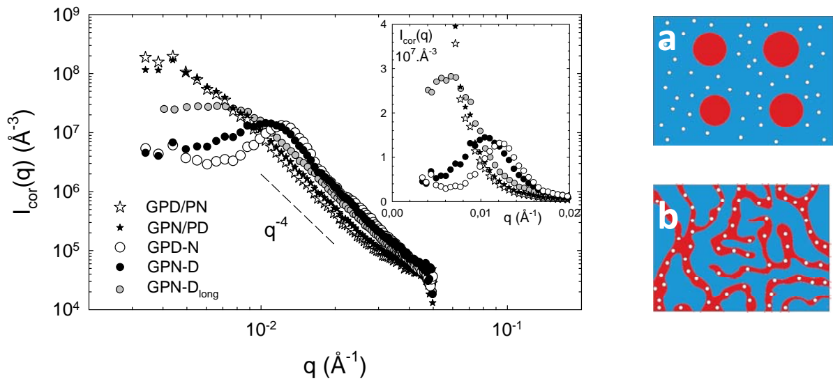
Fig.4. Left: Log-log plot of the normalized* scattered intensity profiles of GPD/PN ( \star ), GPN/PD ( \star ), GPD-N ( \circ ), GPN-D ( \bullet ) and GPN-D long ( \bullet ) at 51.5 °C. The lin-lin plot is given in inset. Right: Micellar (a) and bicontinuous (b) microphase-separated morphologies with PNIPA-rich domains (red), PDMA swollen phase (blue) and chemical cross-linkers (white dots).
