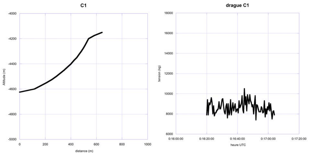
Figure 40: Scheduled bathymetric section for dredge C1.
