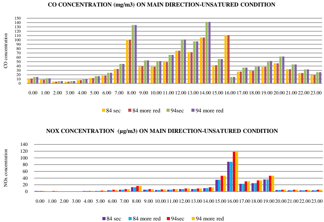
Figure 3: distribution on interval time of CO and NO x concentration on main direction for unsaturated condition
