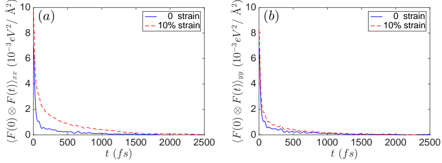
FIG. 5. Time correlation of friction forces along x and y directions for H_2O and graphene.
