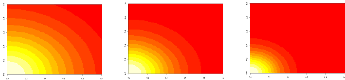
Figure 1. \alpha_\ell^2(\cdot, \cdot) for \ell = 1, 6 and 12 , with \lambda = 2 .
