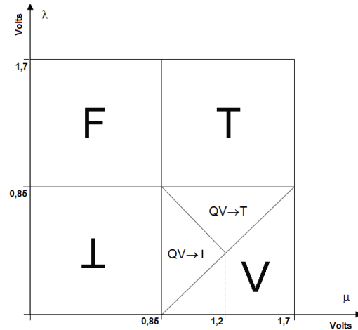
Fig 2. Aspect of the lattice with corresponding voltage levels to the logic states.
