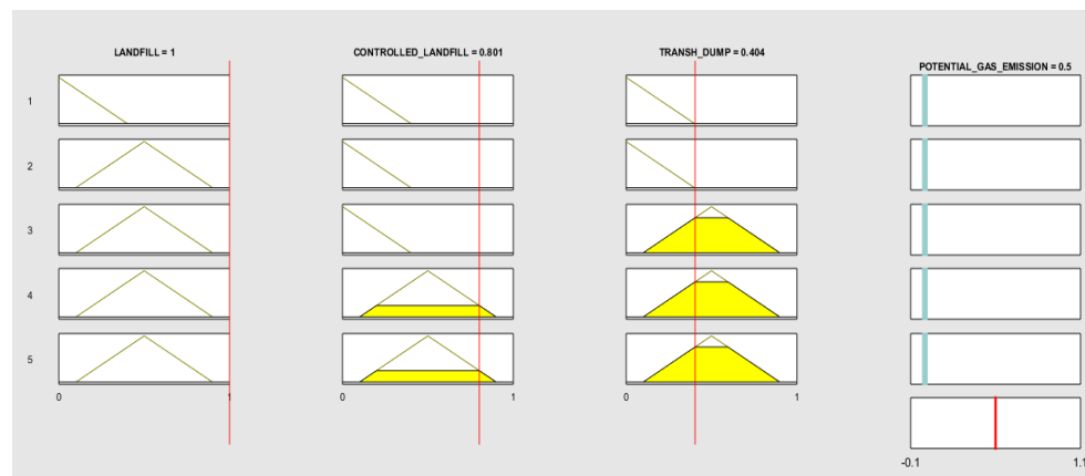
Fig [1] - Simulation result for L_0 ( \text{m}^3/\text{ton} ) with Simulink Fuzzy
