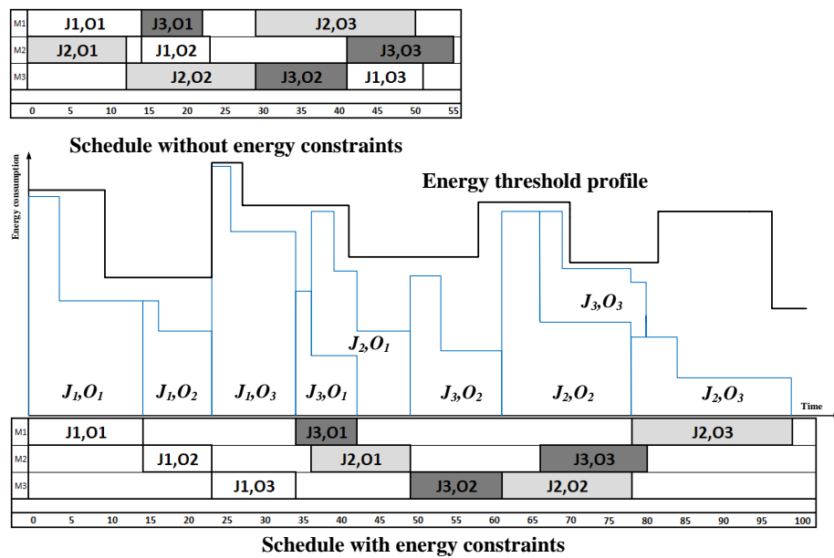
Fig. 3. Impact of the energy threshold on schedules
