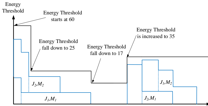
Fig. 2. A Gantt chart of a schedule involving energy threshold variations
