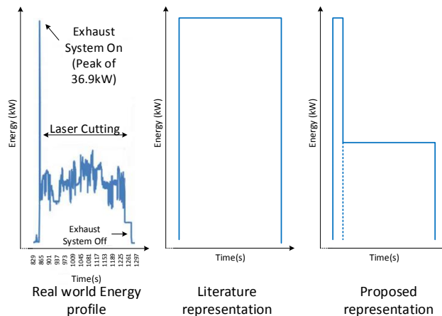
Fig. 1. Power profile of a machine and its representations [1]
