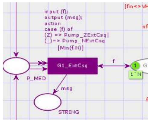
Fig. 4. CPN Model – Pump consequences
