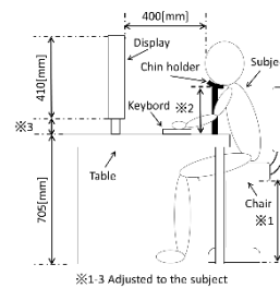
Fig. 5. Experimental layout
