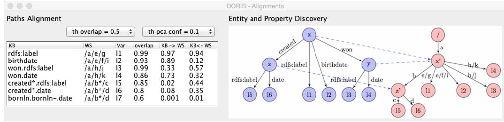
Fig. 3: Paths Alignment - Entity and Property Discovery.
