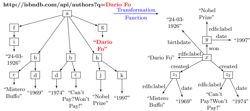
Fig. 2: A call result (left), and its mapping to the KB (right).
