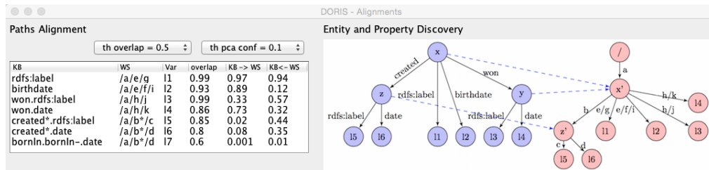
Fig. 3: Paths Alignment - Entity and Property Discovery.
