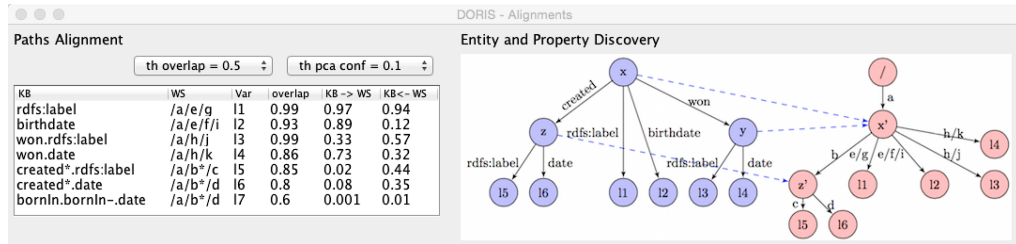
Fig. 3: Paths Alignment - Entity and Property Discovery.
