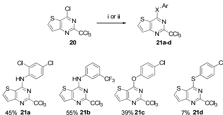
Scheme 5. Synthesis of 4-substituted-2-(trichloromethyl)thieno[3,2- d ]pyrimidine.
