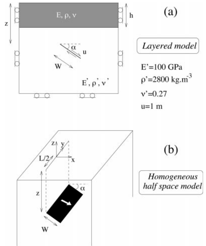
Figure 1. (a) 2-D dislocation model in a layered half-space with an elastic thin layer overlying an elastic half-space (LM). We impose a constant dislocation u=1 m on a fault with a dip angle \alpha , a top depth z=3 km and a width W=10 km. E, \rho, \nu and h are the Young's modulus, the density, the Poisson's ratio and the thickness of the top layer, respectively; E', \rho', \nu' are the Young's modulus, the density and the Poisson's ratio of the half-space, respectively. (b) 3-D dislocation model in a homogeneous half-space (HM) used to invert the coseismic displacements calculated with the LM. W is fixed at 10 km and L/W \sim 3 in the calculations (see text for discussion), while z, u and \alpha are left free.
