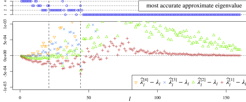
FIG. 10.5. Errors \hat{\lambda}_l^{[j]} - \lambda_l for the geometric approximate eigenvalues induced by the solution \mathbf{v}^* presented in Figure 10.2 (bottom), and indication of the most accurate (smallest absolute error) approximation among \hat{\lambda}_l^{[1]} , \hat{\lambda}_l^{[2]} , \hat{\lambda}_l^{[3]} and \hat{\lambda}_l^{[4]} (top).
