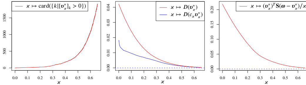
FIG. 11.1. For the MiniBooNE dataset (Gaussian kernel, \omega = \mathbb{1}/N and \mathbf{d} = \mathbb{1} ), graphical representation of the 3 000 first events of the regularisation path related to problem (5.2) for increasing \kappa : number of strictly positive components of \mathbf{v}_\kappa^* as function of \kappa (left); graph of \kappa \mapsto D(\mathbf{v}_\kappa^*) and \kappa \mapsto D(c_\kappa \mathbf{v}_\kappa^*) (middle), and relation between \kappa and the parameter \alpha of the regularised problem (5.1).
