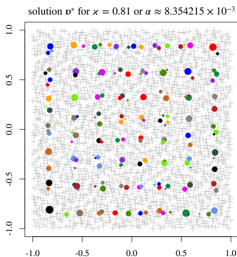
Fig. 8.2: Graphical representation (two-dimensional example) of the solution \mathbf{v}^* to problem (3.2) with \varkappa = 0.81 , or equivalently, to problem (3.1) with \alpha \approx 8.354215 \times 10^{-3} (for \mathbf{d} = \text{diag}(\mathbf{K}) and \boldsymbol{\omega} = \mathbf{1}/N ). The grey crosses represent the points in S and the filled dots are the strictly positive components of \mathbf{v}^* (surface being proportional to v_k^* ).
