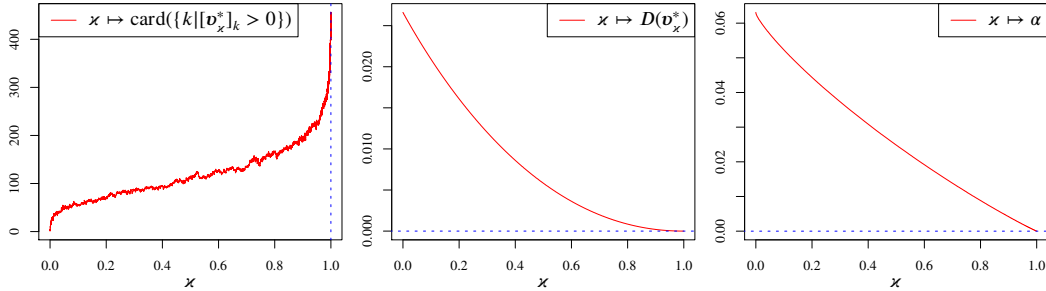
Fig. 8.4: Graphical representation of the 12786 first events of the regularisation path related to problem (3.1) for increasing \varkappa (two-dimensional example): number of strictly positive components in \mathbf{v}_\varkappa^* as function of \varkappa (left); graph of \varkappa \mapsto D(\mathbf{v}_\varkappa^*) (middle), and relation between \varkappa and the regularisation parameter \alpha of problem (3.1) (see Lemma 3.3).
