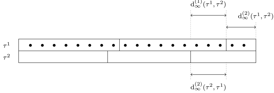
FIG 3. Illustration of the definition of d_\infty^{(i)} , with n = 19 , \tau^1 = [0, 8, 17, 19] and \tau^2 = [0, 7, 14, 19] . In this example, D_{\tau^1} = D_{\tau^2} = 3 . We can compute d_\infty^{(1)}(\tau^1, \tau^2) = d_\infty^{(1)}(\tau^2, \tau^1) = d_\infty^{(2)}(\tau^2, \tau^1) = d_\infty^{(3)}(\tau^1, \tau^2) = 3 and d_\infty^{(2)}(\tau^1, \tau^2) = 2 .
