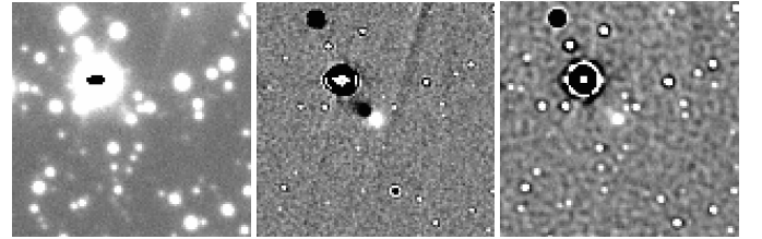
Fig. 2. Example DIA processing of the same original image ( left ), taken on the night of Sep. 20, and showing approximately 26″, or 57 000 km, of the FORS image around the comet. The middle panel shows a DIA subtraction using the best seeing frame from the night of Sep. 20, and removes fainter stars well but demonstrates the negative imprint of the comet from its position in the template frame. The panel on the right uses a template image taken later in the year, but under poorer seeing conditions, resulting in noisier background subtraction and residuals left over from even faint stars, but without any negative comet image. Care was taken to choose the best template image for each night to maximise the number of frames where the comet was well separated from residual sources and any negative imprint.
