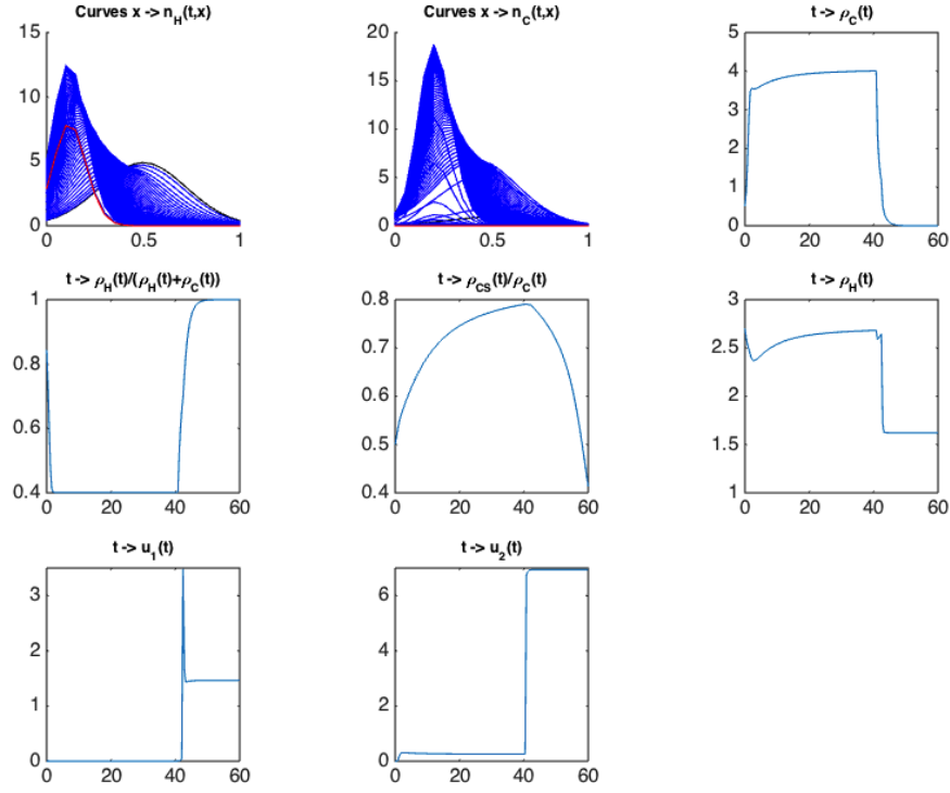
Figure 5: Simulation of (OCP) for T = 60 .
