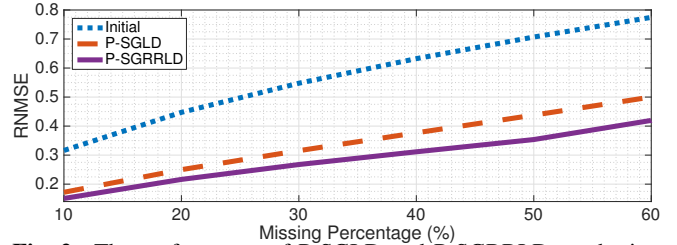
Fig. 2. The performance of P-SGLD and P-SGRRLD on the image restoration problem under the Poisson-NMF model. The initial RMSE is computed by substituting 0 for the missing values.
