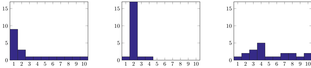
Figure 2. Label histograms for z_n generated by the proposed algorithm for three different pixels.
