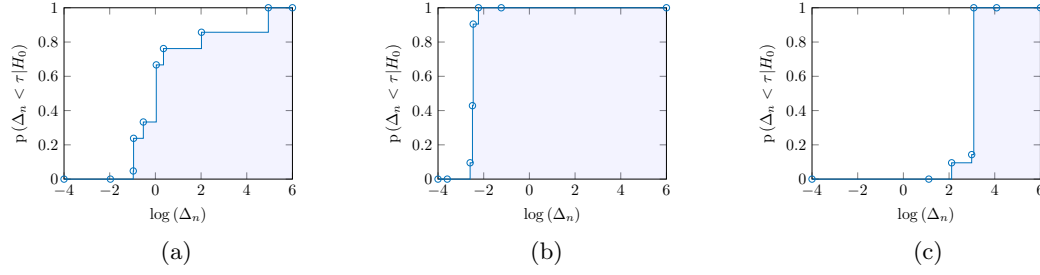
Figure 4. Cumulative distribution p(\Delta_n < \tau|H_0) for three different pixels. Figures 4(a) and 4(b) were obtained from pixels in unchanged areas, while Figure 4(c) was obtained from a pixel in a changed area.
