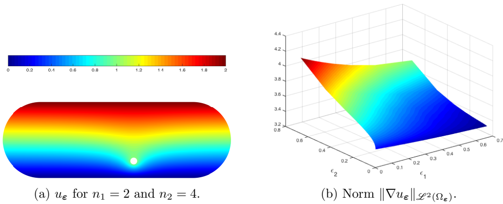
Figure 5: Case g^i = 1 and g^o = x_2 .
