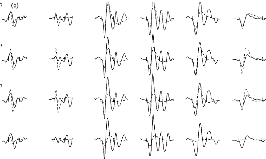
Figure A2. (a) Minimum-misfit solution for the earthquake of 1963 December 16, event 2. (b) The preferred solution for the earthquake of 1963 December 16. The strike of the fault plane is fixed parallel to the local bathymetry. (c) A comparison of different source orientations for the event of 1963 December 16. The display convention is the same as used in Fig. A1. The top line shows the minimum-misfit solution, Line 2 shows our preferred solution. Line 3 is computed with the strike fixed at 147°. Line 4 is the solution of Anderson & Jackson (1987) based on first-motion readings.
