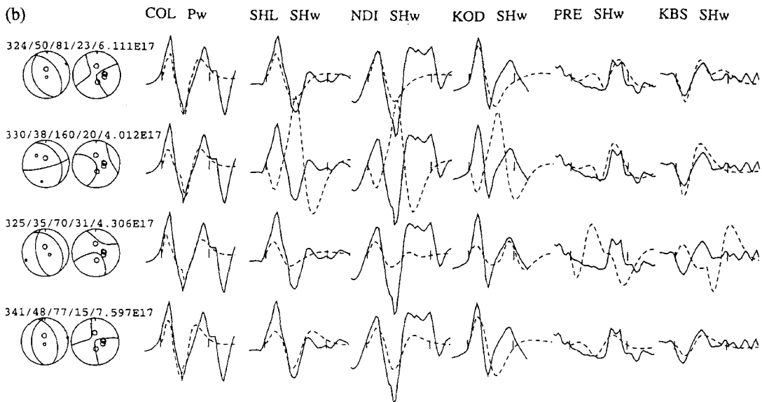
Figure A11. (a) Minimum-misfit solution for the earthquake of 1973 November 4. (b) A comparison of different source mechanisms for the event of 1973 November 4. Line 1 shows the minimum-misfit solution. Line 2 shows one of the two mechanisms proposed by Anderson & Jackson (1987) for this event (the other is close to our minimum-misfit solution). Line 3 shows the mechanism obtained when the dip of the NE-dipping plane is fixed at a shallower value (as seen for events to the north and south) and the other parameters are allowed to vary freely. Line 4 shows the mechanism obtained when the depth is fixed at a shallower value than that obtained in the minimum-misfit solution and the other parameters are allowed to vary freely in the inversion.
