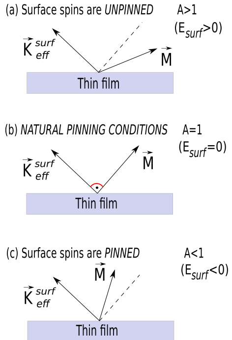
FIG. 2. Schematic representation of three surface spin pinning regimes which prevail in a thin film depending on the configuration of its magnetization \mathbf{M} with respect to the effective surface anisotropy field \mathbf{K}_{eff}^{surf} (see (3.2)). When aligned as in (b), the surface spins do not feel the anisotropy field and A = 1 , which corresponds to their natural freedom. In the configurations (a) and (c) the surface spins are unpinned ( A > 1 ) and pinned ( A < 1 ), respectively, due to the anisotropy field. E_{surf} denotes the surface anisotropy energy density (see (3.3)).
