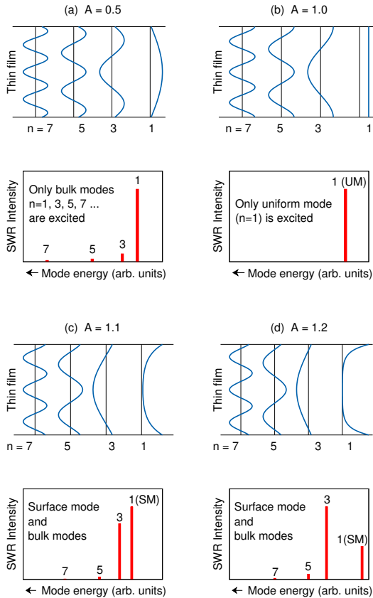
FIG. 3. Profiles of the lowest spin-wave resonance modes (top) and the corresponding SWR spectra (bottom) depicted separately for various values of the surface pinning parameter A ( i.e. for various pinning of the surface spins) within the Surface Inhomogeneity (SI) Model. The spectra only exhibit peaks corresponding to symmetric modes of odd number, n = 1, 3, 5, 7 . The calculations are performed for the case of L = 75 (seventy five layers in the film); UM denotes uniform mode, and SM - surface mode. Two very peculiar effects are observed: firstly, the multi-peak SWR spectrum reduces to a single-peak FMR spectrum at A = 1 , secondly, for A > 1 the spectrum includes a surface-localized resonance peak.
