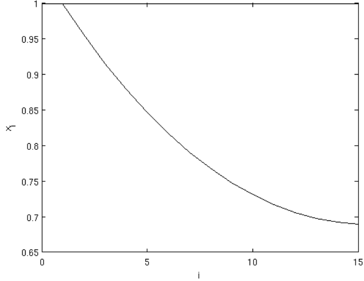
Figure 2: Minimizer of (146).
