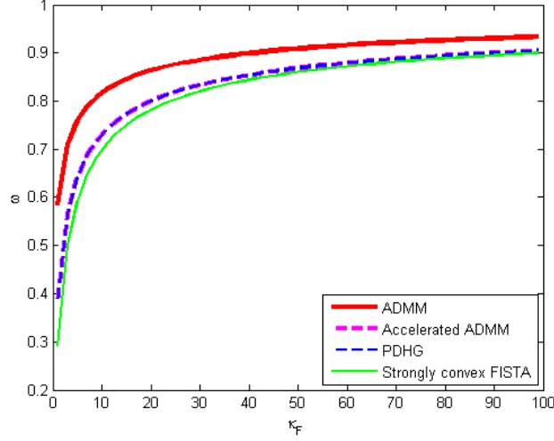
Figure 1: Theoretical rate comparison. In red/thick the unaccelerated ADMM, in magenta/thick dotted the accelerated ADMM, in blue/dotted the overrelaxed PDHG and in green FISTA with constant step.
