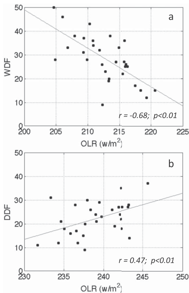
Figure 4. (a) Scatterplot of mean November–March OLR in the northern Tamshiyacu basin (0°S–10°S and 80°W–70°W) versus WDF over the Tamshiyacu basin for the 1980–2009 period. (b) Scatterplot of mean April–August OLR in the southern Tamshiyacu basin (5°S–12.5°S and 87.5°W–70°W) versus DDF over the Tamshiyacu basin for the 1980–2009 period. Regression lines, coefficient of correlations, and p -values are indicated.
