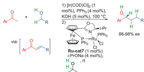
Scheme 18 Sequential ketone alkylation reduction sequence.
