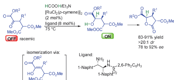
Scheme 15 Lactone synthesis by enantioselective hydrogenative DKR.
