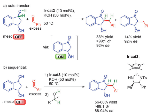
Scheme 21 Ketone alkylation by enantioselective dehydrogenation.
