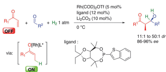
Scheme 34 Enones in enantioselective aldolization.
