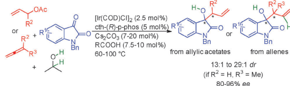
Scheme 38 Use of isatins in enantioselective allylations.
