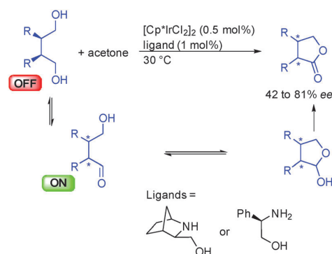
Scheme 14 Enantioselective lactone formation from meso -diols.
