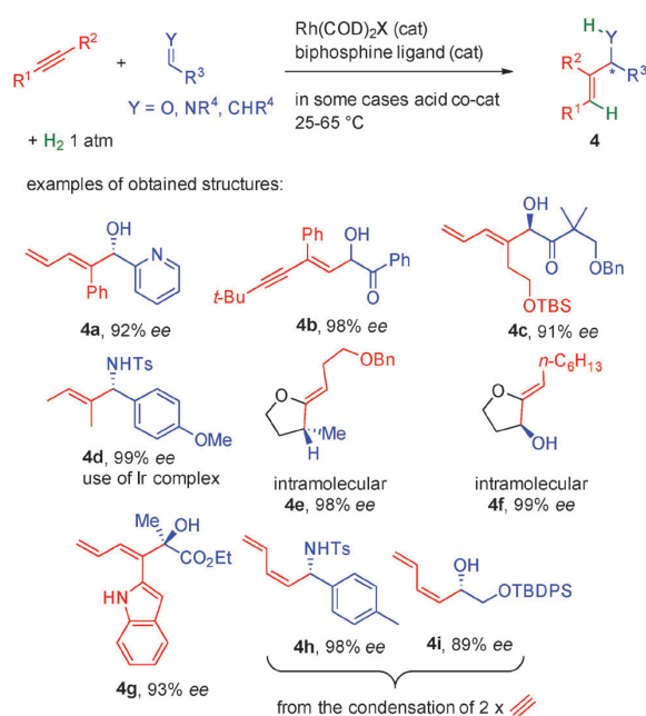
Scheme 33 Alkyne activation by chiral rhodium complexes in the presence of 1 atmosphere of \text{H}_2 .
