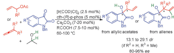
Scheme 38 Use of isatins in enantioselective allylations.
