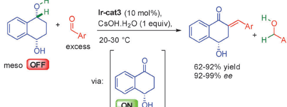
Scheme 22 Dehydrogenative crotonization.
