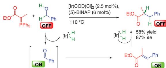
Scheme 19 Hydrogen auto-transfer Wittig type reaction.
