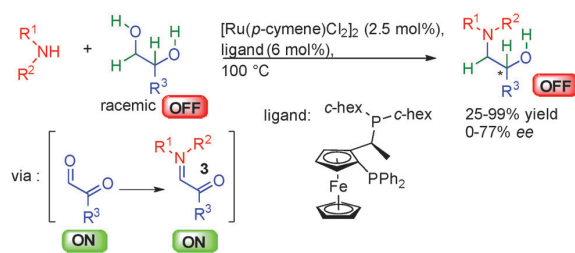
Scheme 27 Amino alcohols synthesis by ruthenium catalysis.
