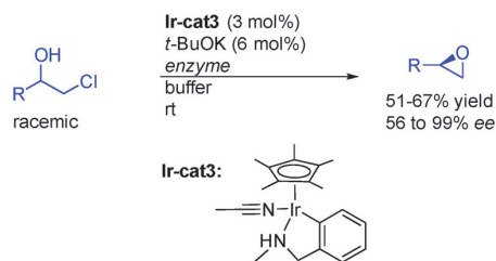
Scheme 8 Direct enantioselective epoxide synthesis.
