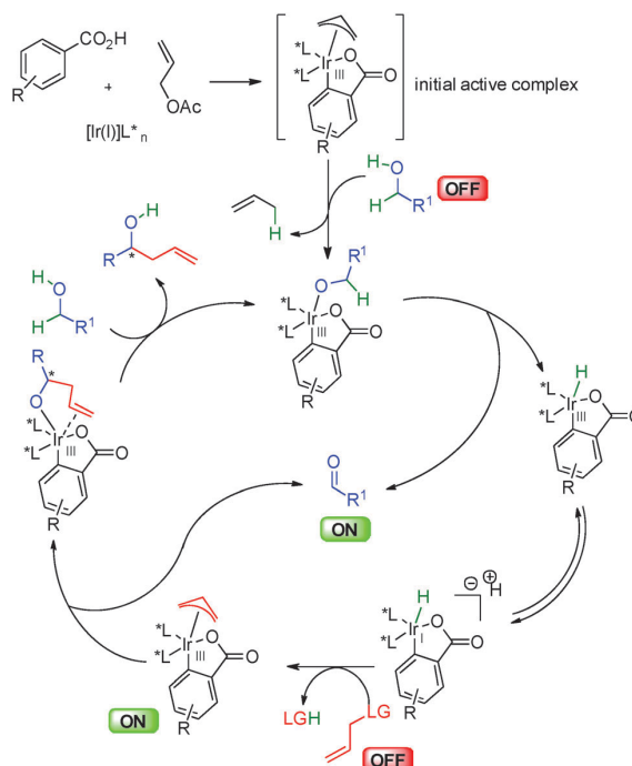
Scheme 36 General mechanism of hydrogen mediated allylation.
