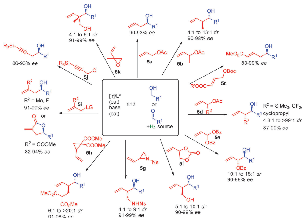
Scheme 35 Scope of the hydrogen mediated allylation.
