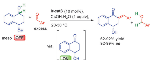
Scheme 22 Dehydrogenative crotonisation.
