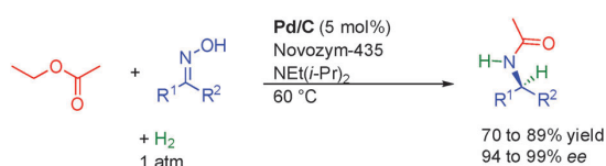
Scheme 10 Preparation of chiral amines from ketoximes.
