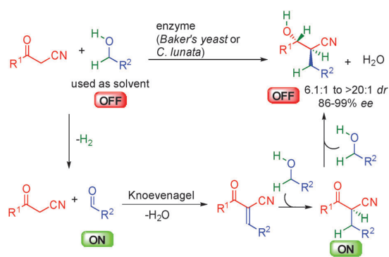
Scheme 17 Enzyme catalyzed \alpha -cyano-ketone alkylation-reduction sequence.
