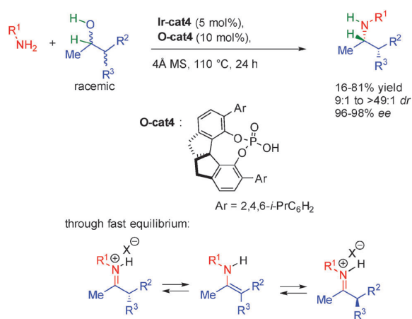
Scheme 29 Amino-alcohols synthesis by DKR through borrowing hydrogen.
