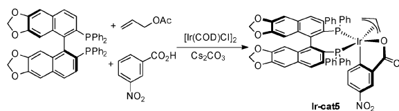
Scheme 37 Example of active iridium complex formation.
