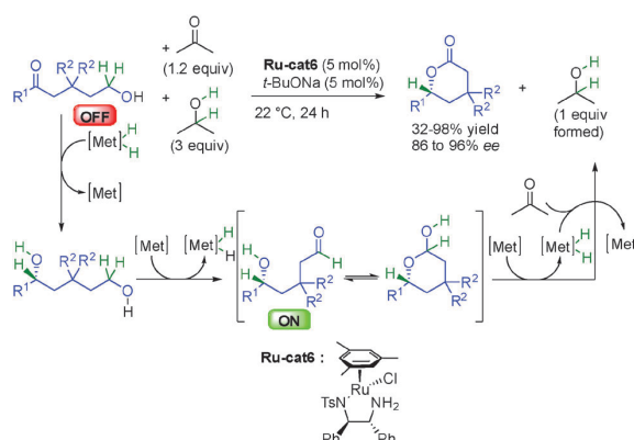
Scheme 16 Enantioselective lactone synthesis by multiple hydrogen transfers.
