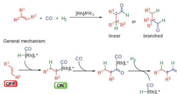
Scheme 31 General pathway for enantioselective hydroformylation.
