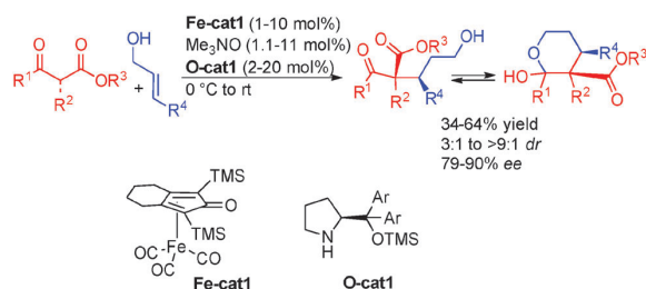
Scheme 24 Enantioselective addition of keto-esters to allylic alcohols.
