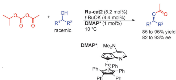
Scheme 9 Dual organocatalytic/ruthenium catalysis for DKR of alcohols.
