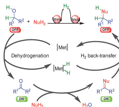
Scheme 2 General concept of borrowing hydrogen.
