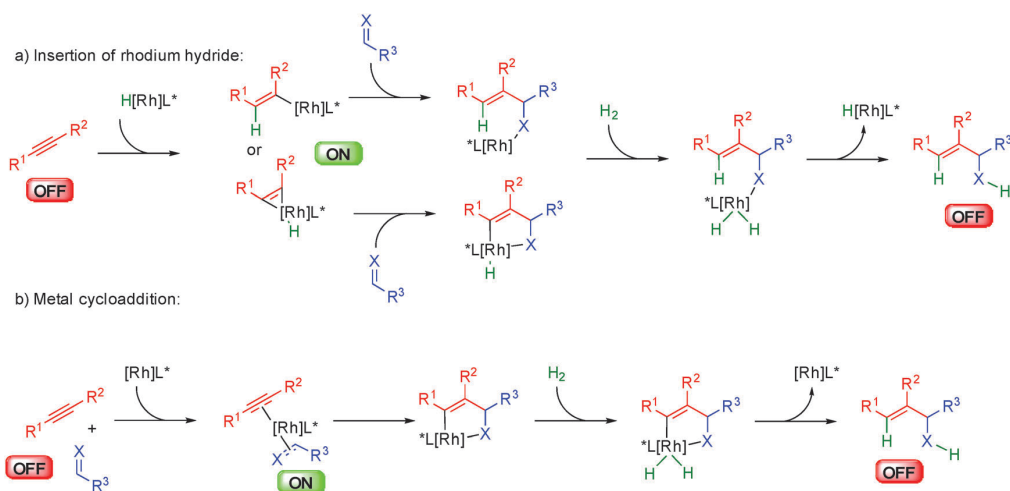
Scheme 32 General mechanism for hydrometallation of alkynes.
