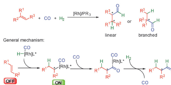
Scheme 31 General pathway for enantioselective hydroformylation.
