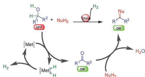
Scheme 3 General concept of dehydrogenative activation.
