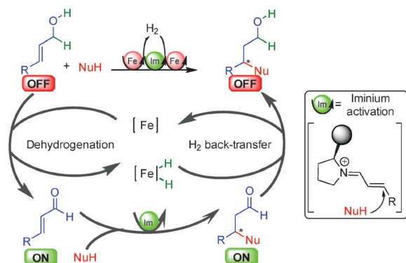
Scheme 23 Concept of the dual allylic alcohols functionalization.
