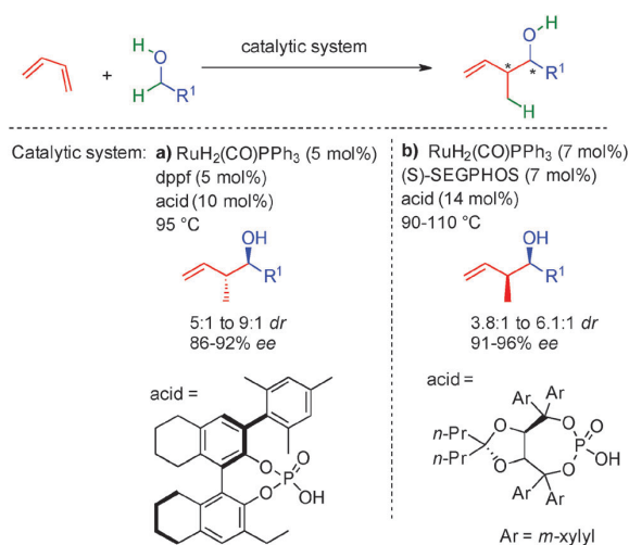
Scheme 41 Diastereodivergent allylation using butadiene.
