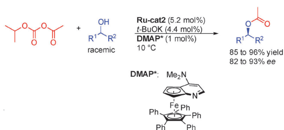
Scheme 9 Dual organocatalytic/ruthenium catalysis for DKR of alcohols.
