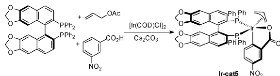
Scheme 37 Example of active iridium complex formation.
