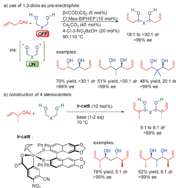
Scheme 39 Direct enantioselective synthesis of 1,3-diols.
