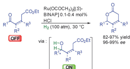
Scheme 12 Enantioselective lactone formation from keto-esters.
