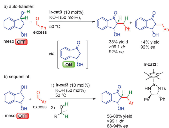
Scheme 21 Ketone alkylation by enantioselective dehydrogenation.
