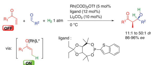
Scheme 34 Enones in enantioselective aldolization.
