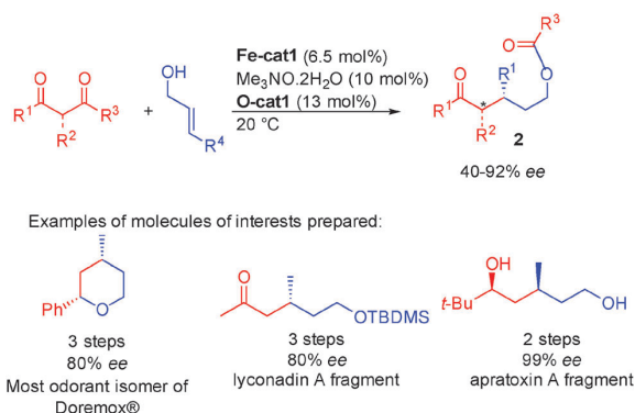
Scheme 25 Borrowing hydrogen cascade fragmentation.
