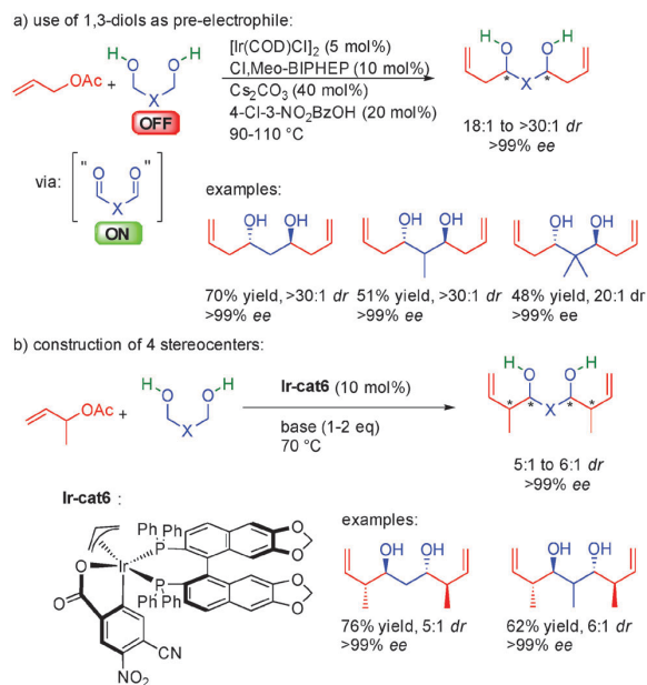
Scheme 39 Direct enantioselective synthesis of 1,3-diols.
