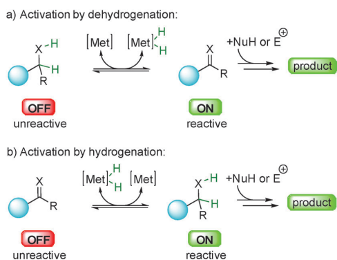
Scheme 1 General concept of OFF \leftrightarrow ON activation by hydrogen transfer.
