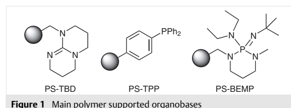
Figure 1 Main polymer supported organobases
