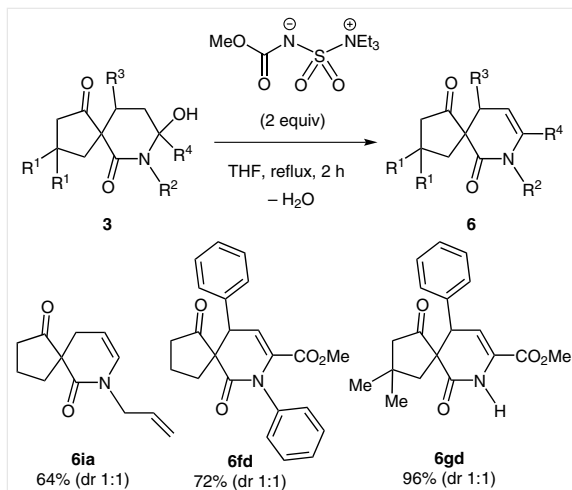
Scheme 5 Dehydration of spirohemiaminals 3
