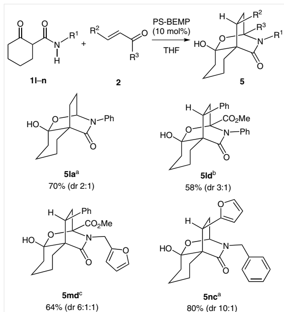
Scheme 4 Formation of polycyclic hemiacetals 5 from six-membered alicyclic 1,3-ketoamides 11-n . a Reaction conducted at 55 °C for 24 h. b Reaction conducted at r.t. for 30 h. c Reaction conducted at r.t. for 5 h.
