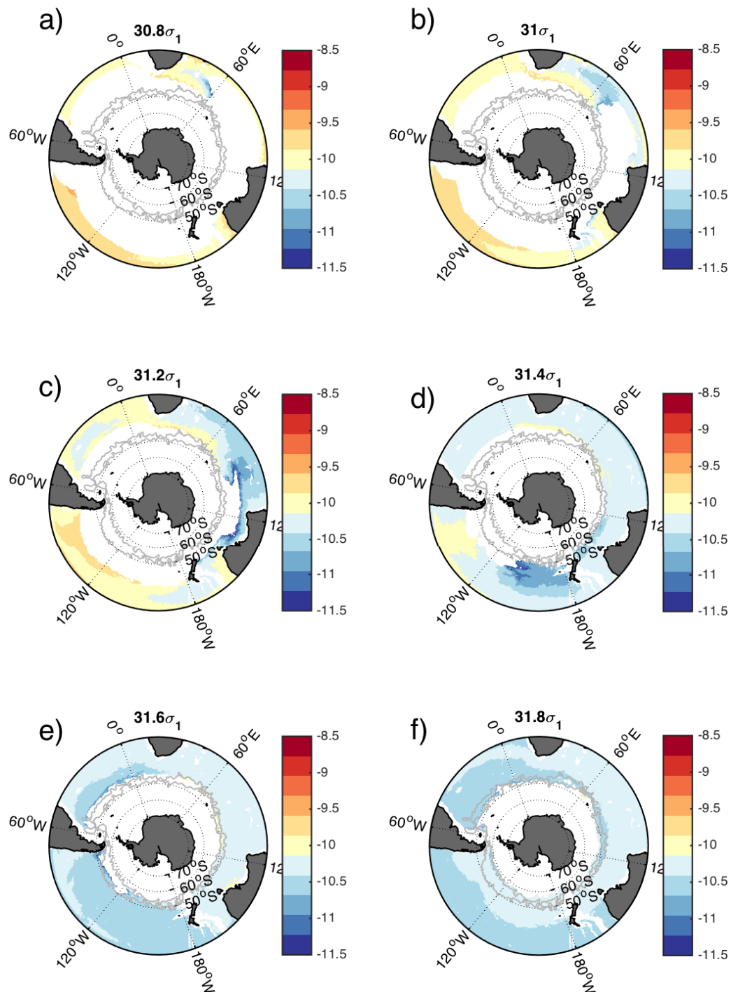
Figure 1. Annual mean potential vorticity (1/ms, log 10 scale) in BASSOON after the 10 year spin-up period, projected onto \sigma_1 potential density surfaces ( \text{kg/m}^3 ). The two solid lines are the 90 Sv and 130 Sv contours of the annual mean barotropic streamfunction after the 10 year spin-up period ( 1 \text{ Sv} = 10^6 \text{ m}^3/\text{s} ).
