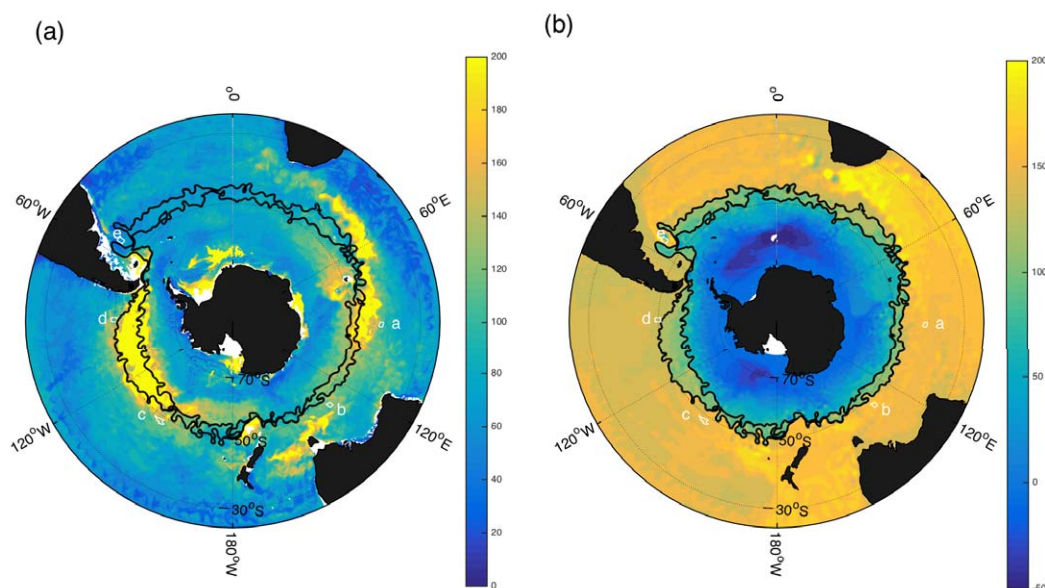
Figure 3. The size and placement of the initial tracer patches, indicated by white contours and letters. The color scales show (a) JJA mixed layer depth [m], calculated by integrating the stratification d\rho/dz from the surface down to z_{ml} , where \Delta\rho = \rho(z_{ml}) - \rho(z=0) = 0.03 \text{ kg/m}^3 , and (b) annual mean vertically integrated transport (Sv). The two solid lines are the 90 Sv and 130 Sv contours of the annual mean barotropic streamfunction after the 10 year spin-up period.
