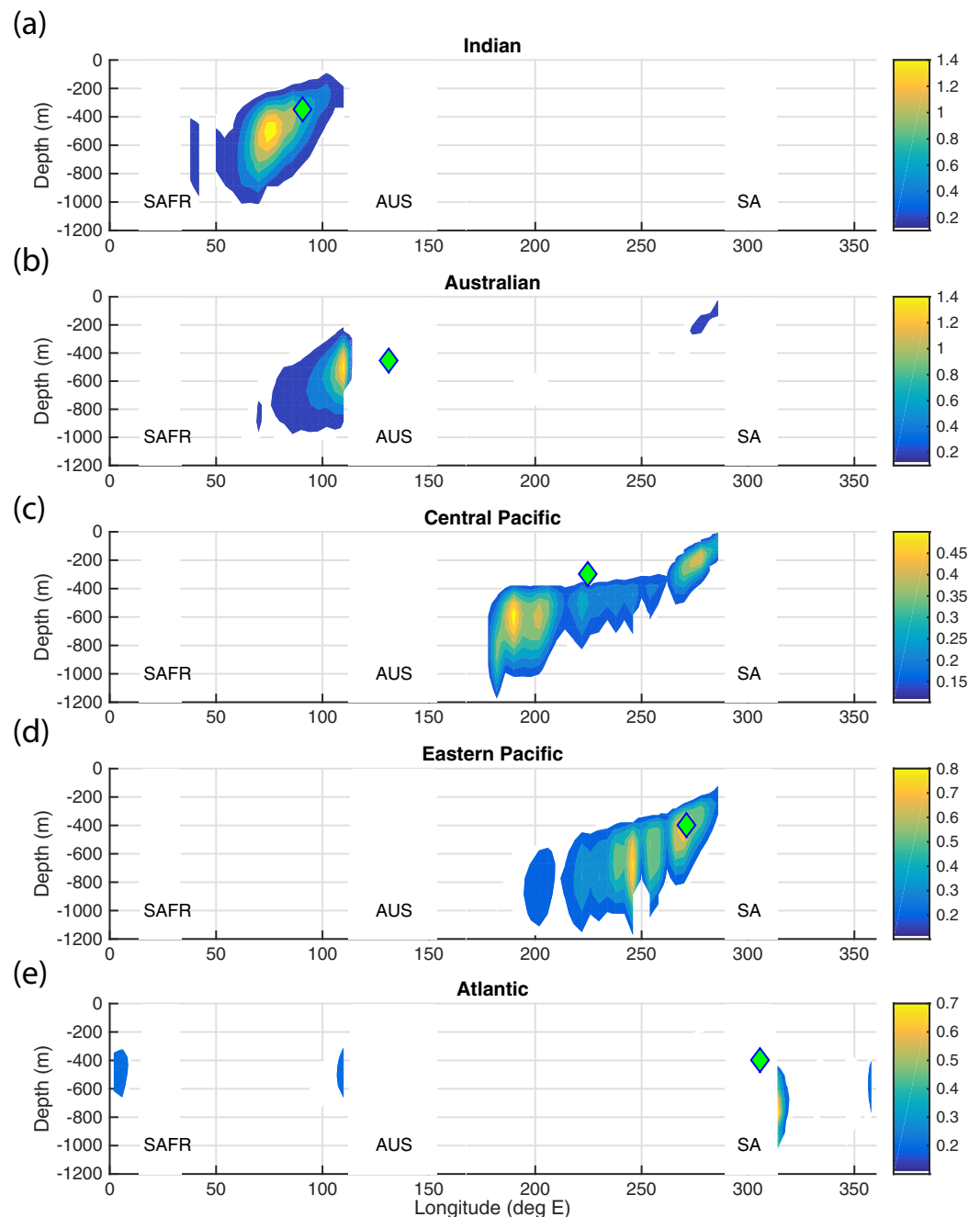
Figure 11. Spatial distribution of the cumulative tracer removed by the sponge at the northern boundary ( 24.7\text{--}26.5^\circ\text{S} ) 50 years into the experiment, as a fraction of the initial tracer. Shown from top to bottom are the (a) Indian, (b) Australian, (c) Central Pacific, (d) Eastern Pacific, and (e) Atlantic tracer advection experiments. Approximate initial tracer locations are indicated by green diamonds. Removal percentages have been summed onto a grid with 90 points in the horizontal and 42 points in the vertical for clarity.
