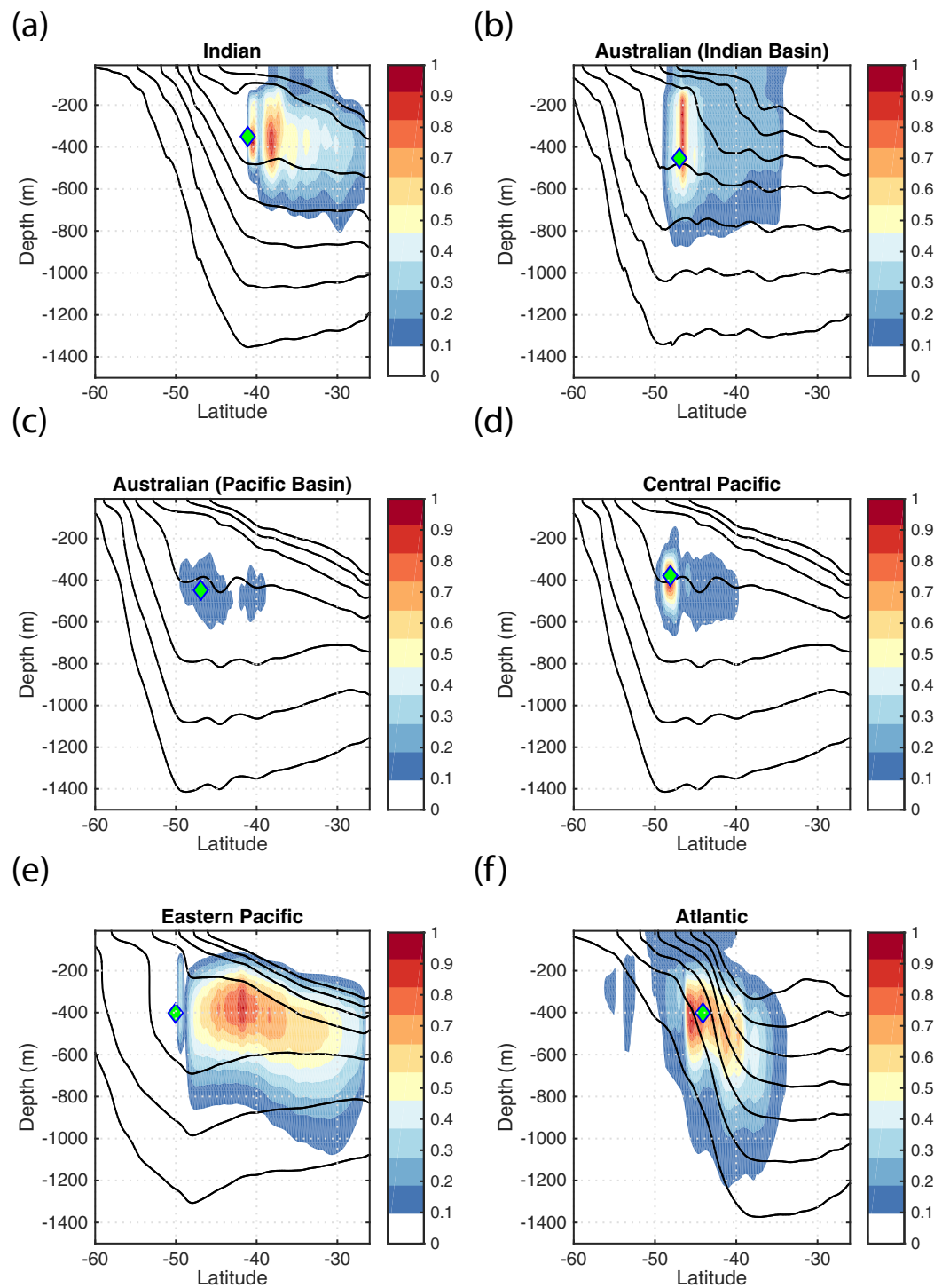
Figure 7. Tracer distribution histograms for each of the 50 year tracer advection experiments. Each color map has been scaled by the maximum concentration of each tracer, which is different for each experiment. Initial locations are indicated by green diamonds. The black solid lines are \sigma_1 potential density surfaces ( 30.8\text{--}32.0\text{ kg m}^{-3} , every 0.2\text{ kg m}^{-3} ). The tracer concentrations and potential densities are averaged in 10^\circ wide swaths about the longitudes of the tracer centers of mass. (b) Only includes Australian tracer located in the Indian basin, and (c) only includes Australian tracer located in the Pacific basin.
