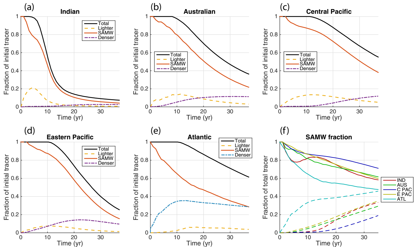
Figure 9. (a–e) Time series of the proportion of each mode water tracer that is less dense than SAMW (“lighter,” <31.0\sigma_t ), in the SAMW density range ( 31.0\text{--}31.8\sigma_t ), or more dense than SAMW ( >31.8\sigma_t ), relative to the initial amount of tracer used in each experiment. The initial tracer locations are shown in Figure 6f. (f) The SAMW fraction of each mode water tracer (solid lines) and the fraction denser than SAMW (dashed lines), relative to the total amount of remaining tracer in the model domain.
