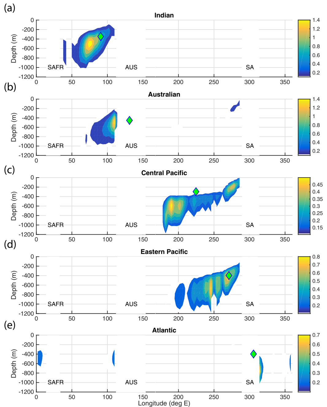
Figure 11. Spatial distribution of the cumulative tracer removed by the sponge at the northern boundary (24.7–26.5°S) 50 years into the experiment, as a fraction of the initial tracer. Shown from top to bottom are the (a) Indian, (b) Australian, (c) Central Pacific, (d) Eastern Pacific, and (e) Atlantic tracer advection experiments. Approximate initial tracer locations are indicated by green diamonds. Removal percentages have been summed onto a grid with 90 points in the horizontal and 42 points in the vertical for clarity.
