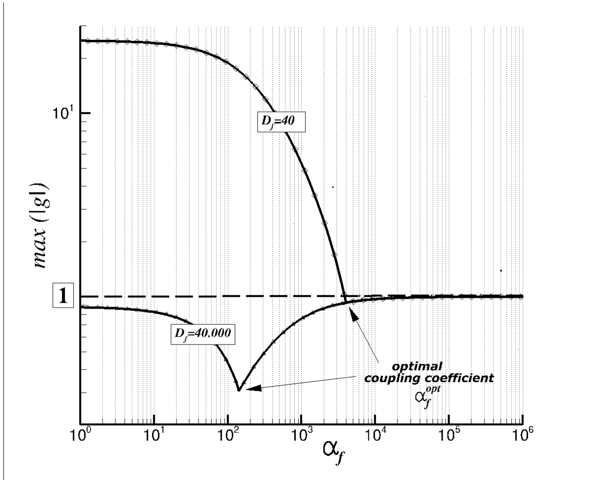
Figure 1: Amplification factor for D_f = 40 & D_f = 40.000 Dirichlet-Robin procedure
