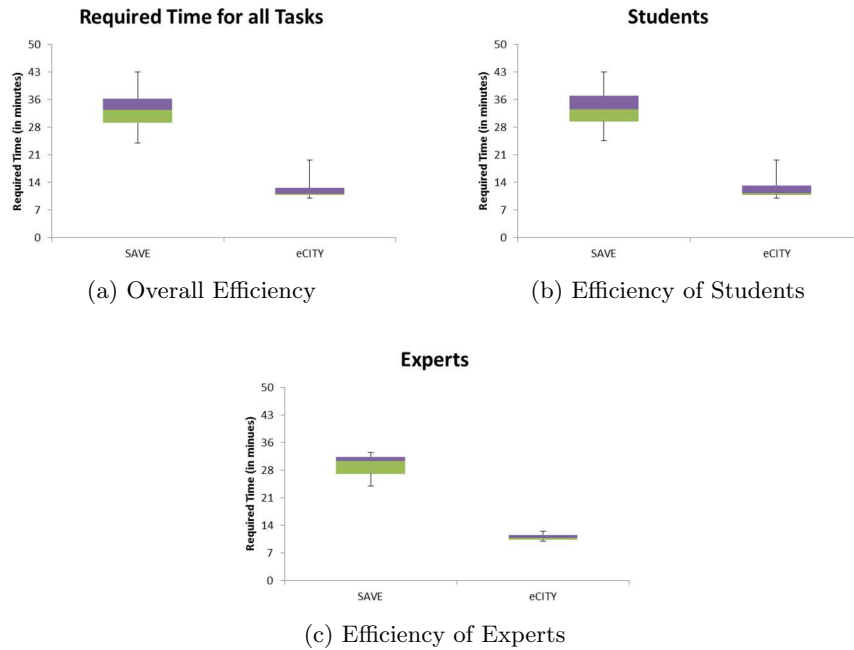
Fig. 4. Efficiency Box-plots (x-axis: left SAVE, right eCITY, y-axis: required time in minutes)
