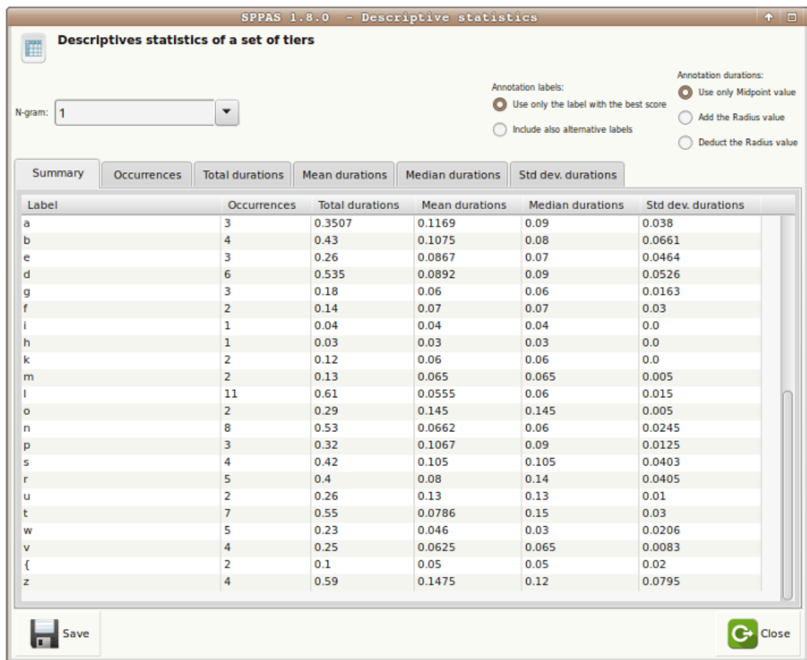
Figure 5.2: Descriptive statistics
