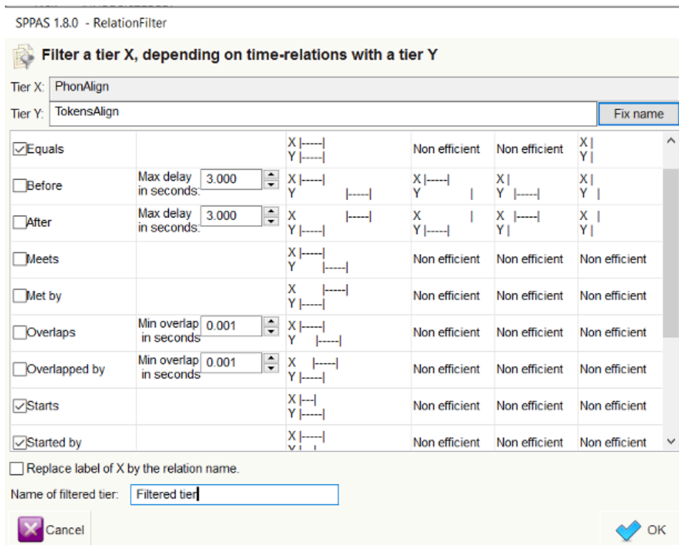
Figure 6.13: DataFilter: RelationFilter frame
