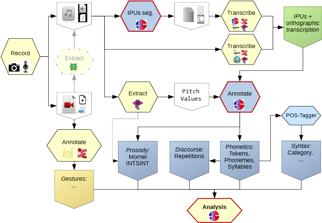
Figure 4.1: Annotation methodology
