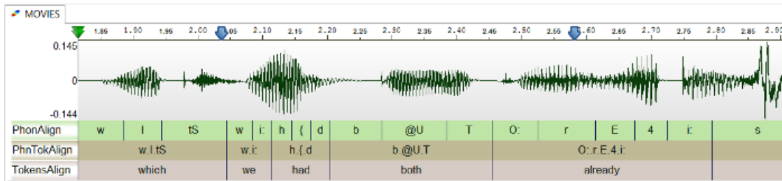
Figure 3.11: SPPAS alignment output example
