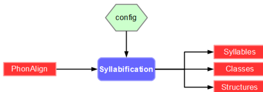
Figure 3.17: Syllabification workflow
