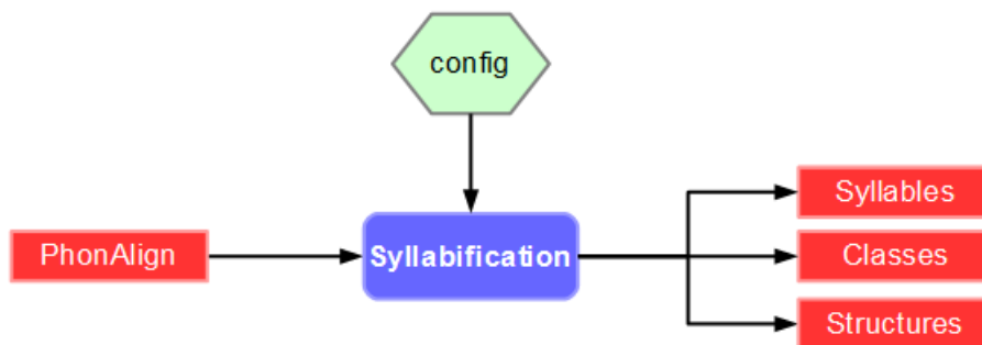
Figure 3.18: Syllabification workflow
