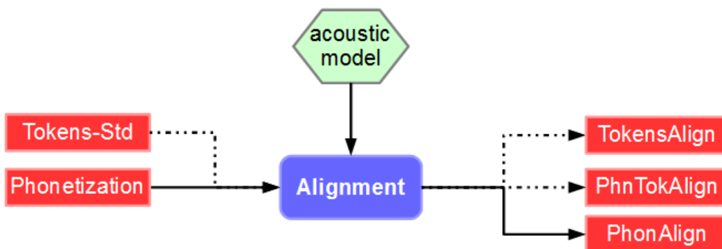
Figure 3.16: Alignment workflow
